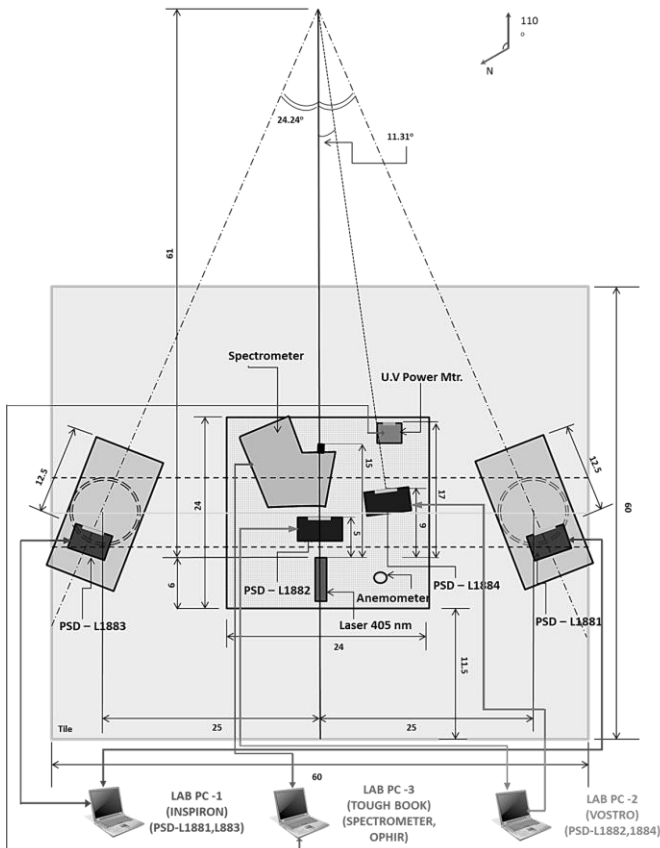
Figure 5: Schematic of the set up during field experiment for monitoring free air stream velocity.
