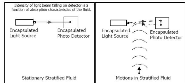
Figure 2: Schematic description of the working principle of photonics system for monitoring stratified fluid motions.
